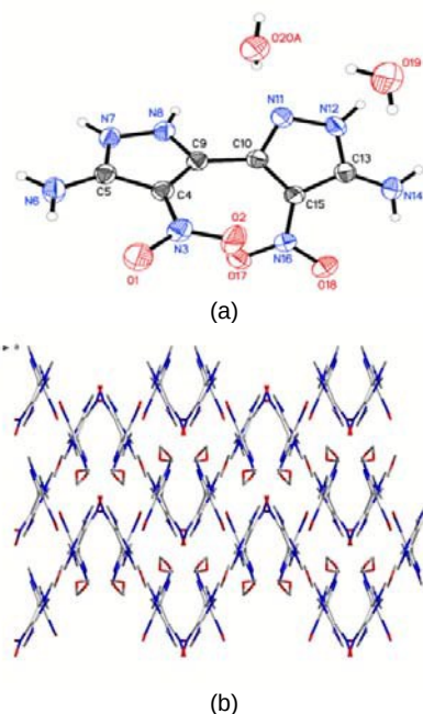
Fig. 2 (a) Molecular structure of 7 •2H 2 O solvate by thermal displacements ellipsoids with 50% probability. (b) A view of the packing diagram along the b axis
