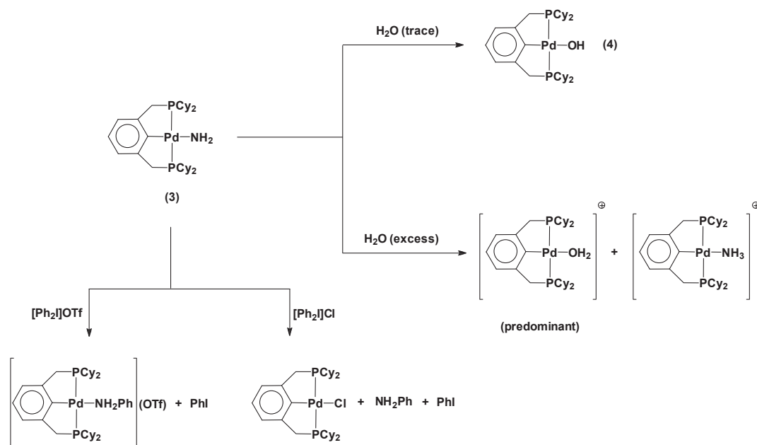
Scheme 4. Reactions of 3 with \text{H}_2\text{O} and [\text{Ph}_2\text{I}]\text{X} ( \text{X} = \text{OTf}, \text{Cl} ).
