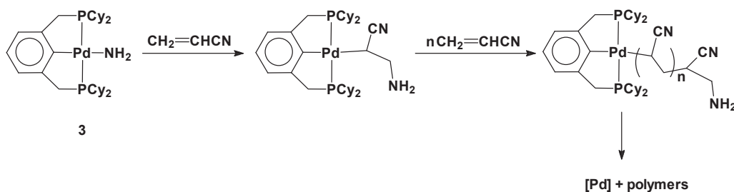
Scheme 6. Reaction of 3 with acrylonitrile.
