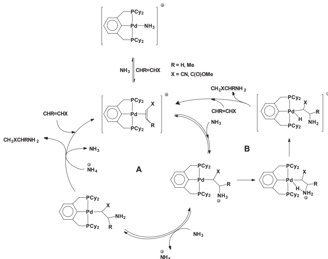
Scheme 7. Plausible reaction pathways for the observed hydroamination of olefins with ammonia in the presence of \text{Pd}(2,6-(\text{Cy}_2\text{PCH}_2)_2\text{C}_6\text{H}_3)(\text{OTf}) , involving an aminoalkyl \text{Pd}(\text{II}) species (pathway A) or a \text{Pd}(\text{IV}) hydride (pathway B).
