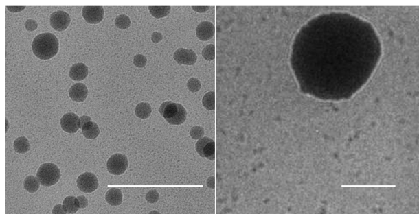
Figure 7. Cryo-TEM pictures from solutions of 4.5 mM Mn(IV)-OH-PFOM and 70 mM of MCl. M = K (left), and Cs (right) at 60 °C. Scale bar is 200 nm, dark is high contrast, ie W.
