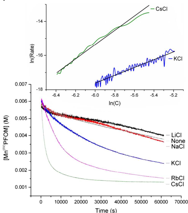
Figure 5. Bottom: Profiles of the reaction of 4.5 mM Mn(IV)-OH-PFOM in the presence of 70 mM of MCl (M=Li, Na, K, Rb or Cs) at 80 °C. KF yielded essentially the same result as KCl and KBr was oxidized to Br 2 . Top: \ln/\ln plots of the reaction rates versus concentration generated from the reaction profiles. Experimental data (colored) and linear fit (black). Slope: KCl = 2.2; CsCl = 4.1. Note that the noise in the UV-vis measurement is amplified in the data manipulation.
