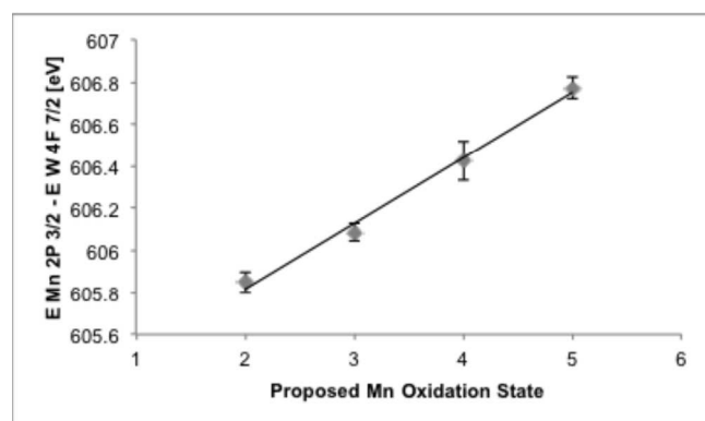
Figure 3. Corrected binding energies of Mn 2p^{3/2} as a function of the oxidation state of manganese.
