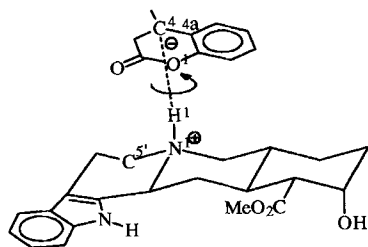
Scheme 5. The ion pair 10 , in which 4\text{-H}^+ protonates 8^- .
