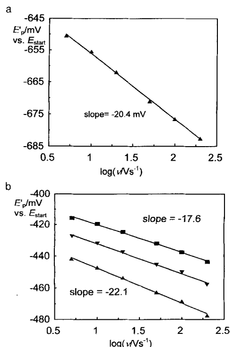
Figure 12. Peak potential dependence of the first derivative of the signal on the sweep rate at different concentrations of HCl measured by LSV. C^0(\text{I}) = 1 mM in MeOH/ \text{H}_2\text{O} (1/1) (0.2 M \text{Et}_4\text{NBr} ), T = 21^\circ\text{C} , Hg/Pt electrode. a) C^0(\text{HCl}) = 0 mM; b) C^0(\text{HCl}) = 10 mM (▲), 20 mM (▼), and 40 mM (■).
