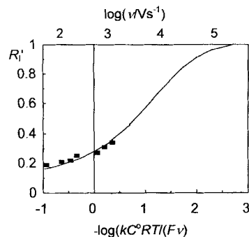
Figure 8. Fit of experimental values of R_1' vs. \log v measured by DCV ( E^0 - E_{sw} = 0.2 V) for 1 . C^0(\mathbf{1}) = 0.5 mM, in MeOH/H _2 O (1/1) (0.2 M Et _4 NBr) to theoretical data for the mechanism described in Scheme 3 with rate-determining dimerization. T = 21^\circ C, Hg/Pt electrode.
