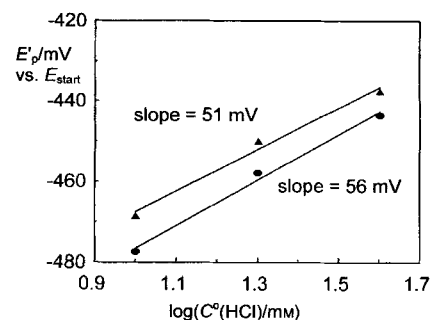
Figure 13. Peak potential dependence of the first derivative of the signal on the concentration of HCl, C^0(\text{HCl}) = 10 , 20 and 40 mM, at two scan rates, v = 100 (▲) and 200 \text{Vs}^{-1} (●), determined by LSV. C^0(\text{I}) = 1 mM in MeOH/ \text{H}_2\text{O} (1/1) (0.2 M \text{Et}_4\text{NBr} ), T = 21^\circ\text{C} , Hg/Pt electrode.
