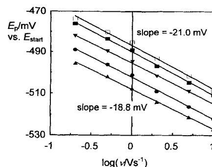
Figure 6. Dependence of peak potential on the sweep rate, \nu = 0.2\text{--}10 \text{Vs}^{-1} , determined by LSV at C^0(\mathbf{1}) = 0.5 mm ( \Delta ), 1 mm ( \bullet ), 2 mm ( \blacktriangledown ), 4 mm ( \blacksquare ), and 8 mm ( \square ) in MeOH/ \text{H}_2\text{O} (1/1) (0.2 M \text{Et}_4\text{NBr} ), T = 21^\circ\text{C} , Hg/Pt electrode. The values of dE_p/d\log \nu are all in the range -18.8 to -21.0 mV/decade.
