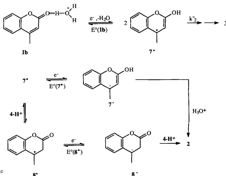
Scheme 4. Mechanism of the cathodic reduction of 1 to 2 and 3 in acidic MeOH/ \text{H}_2\text{O} .
