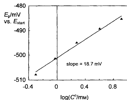
Figure 7. Dependence of peak potential on the concentration of 1 . C^0(\mathbf{1}) = 0.5 – 8 mM, determined by LSV at v = 1 Vs ^{-1} in MeOH/H _2 O (1/1) (0.2 M Et _4 NBr), T = 21^\circ C, Hg/Pt electrode.
