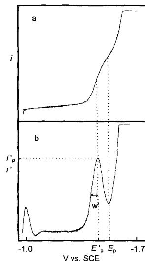
Figure 10. The current (a) and the first derivative (b) of the current for a linear potential sweep in the range -1.0 to -1.7 V vs. SCE at v = 100 Vs ^{-1} on a 1 mM solution of 1 in MeOH/H _2 O (1/1) (0.2 M Et _4 NBr) upon addition of 10 mM HCl. T = 21^\circ C, Hg/Pt electrode.
