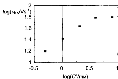
Figure 1. Dependence of the value of v_{0.5} determined by DCV on the concentration of 1 . C^0(\mathbf{1}) = 0.5, 1, 2, 4 and 8 mM, in DMF (0.1 M Et 4 NBr), E^0 - E_{\text{sc}} = 0.2 V, T = 21^\circ\text{C} , Hg/Pt electrode.
