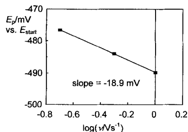
Figure 2. Dependence of peak potential on sweep rate, v = 0.2 – 1 Vs -1 , determined by LSV. C^0(\mathbf{1}) = 8 mM in DMF (0.1 M Et 4 NBr), T = 21^\circ\text{C} , Hg/Pt electrode.
