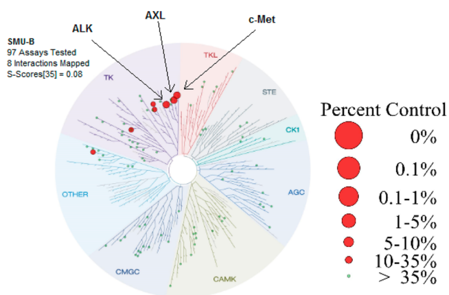
Figure 6. Kinase dendrogram of compound 5b (SMU-B) at [drug] = 100 nM in DiscoverX's scanEDGE SM against 97 wild-type and mutant kinases.
