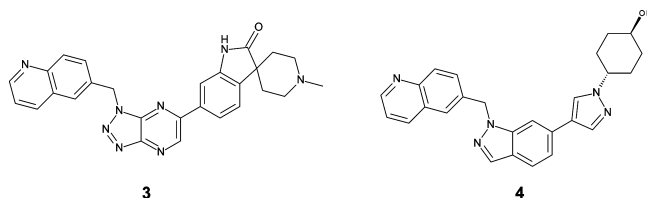
Figure 2. Compounds 3 22 and 4 23 as c-Met inhibitors.
