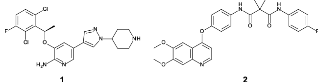
Figure 1. Crizotinib ( 1 ) and Cabozantinib ( 2 ).
