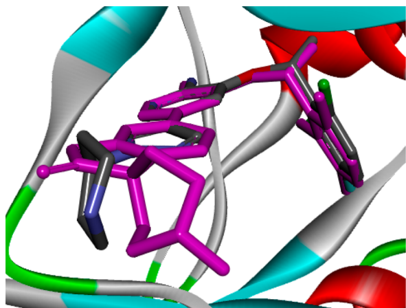
Figure 4. Overlay of Crizotinib (magenta) and compound 5b (gray) in c-Met kinase domain (PDB code: 2WGJ).
