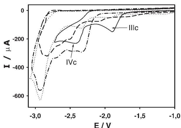
Figure 7. Time evolution of the CVs of the 1a /PhN 2 H 3 system. Scan rate: 0.2\text{ Vs}^{-1} . 1a : 7.83\text{ mM} ; PhN 2 H 3 : 19.0\text{ mM} . Scanned solutions were prepared by dilution (with 0.1\text{ M NaClO}_4 , DMF) of a stock 1a -PhN 2 H 3 -DMF solution, as detailed in the text. (—): CV scanned immediately after stock solution preparation ( t=0 ), (---): t=48\text{ h} , (- · -): t=364\text{ h} , (· · ·): CV of a 7.51\text{ mM} 4a solution in 0.1\text{ M NaClO}_4 , DMF
