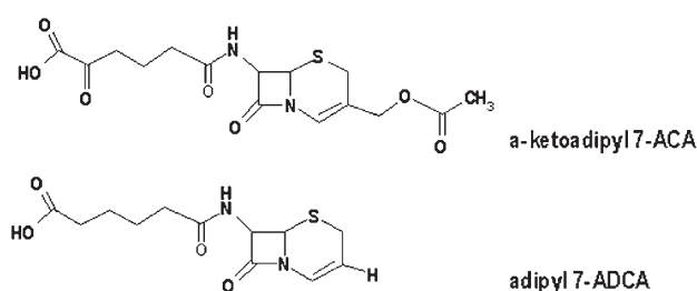
Scheme 1. Adipoyl-7-ADCA and 2-oxoadipoyl-7-ACA structures. The difference between the two substrates is mainly in their aliphatic side-chains. In the case of 2-oxoadipoyl-7-ACA, the side chain has a carbonyl group in the \alpha -carbon, whereas the adipoyl-7-ADCA does not have this carbonyl group in its side-chain. The differences in the C-3 modifications between the two substrates do not translate in a different way to the interaction of both substrates with the binding pocket of the enzyme.
