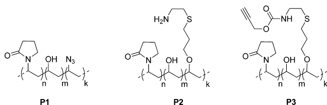
Figure 2. Functionalized copovidone with azide P1 , amino P2 , and alkyne P3 pendant groups.
