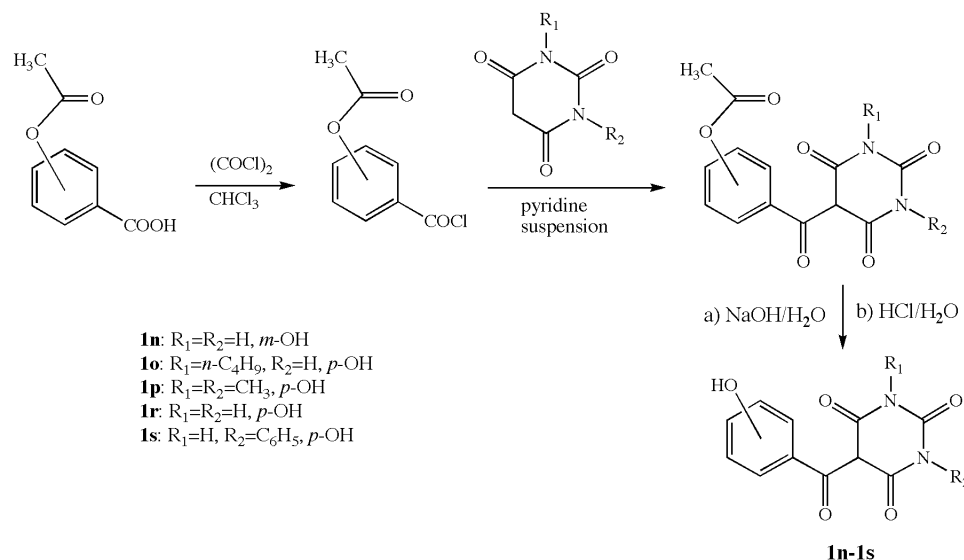
Synthetic pathway for preparation hydroxybenzoylbarbiturates 1n-1s .
