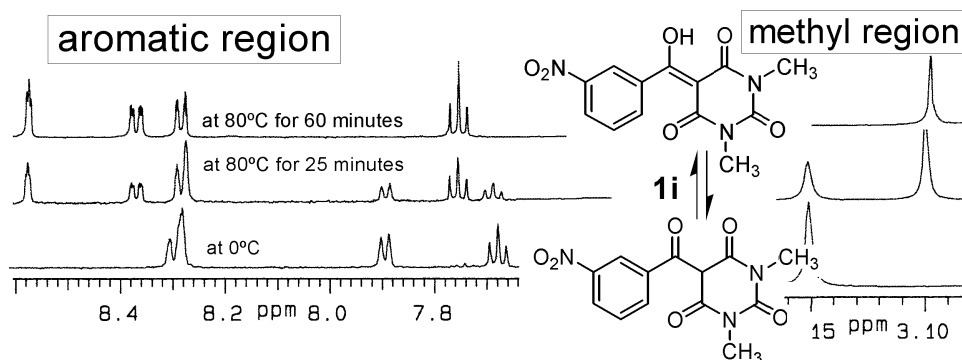
Figure 1. The NMR following of thermal induced transformation of the keto form of 1i into the enol form in \text{DMSO}-d_6 at 80 °C.
