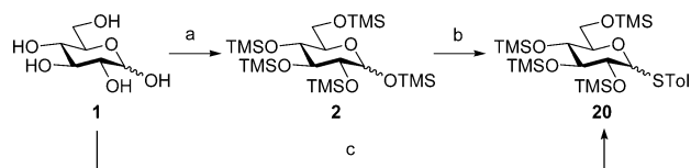
Scheme 4. MW-Assisted One-Pot Thioglycoside Formation a
