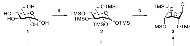
Scheme 2. MW-Assisted 1,6-Anhydroglucose Formation a
