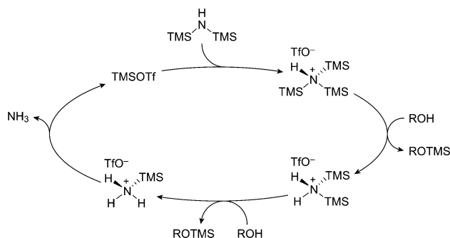
Scheme 1. Proposed Catalytic Cycle for the TMSOTf-Mediated Alcohol Silylation by HMDS
