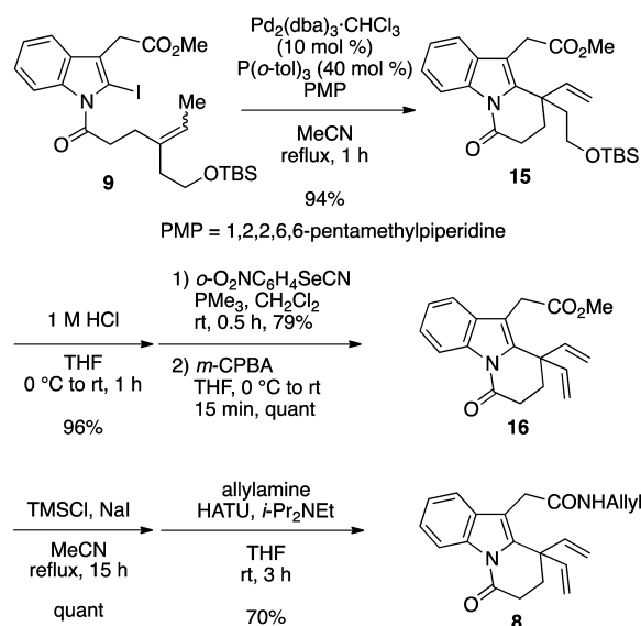
Scheme 3. Construction of Quaternary Carbon Center and Conversion to Indole-3-acetamide 8
