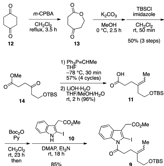
Scheme 2. Preparation of N -Acylindole 9
