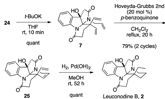
Scheme 6. Total Synthesis of Leuconodine B (2)
