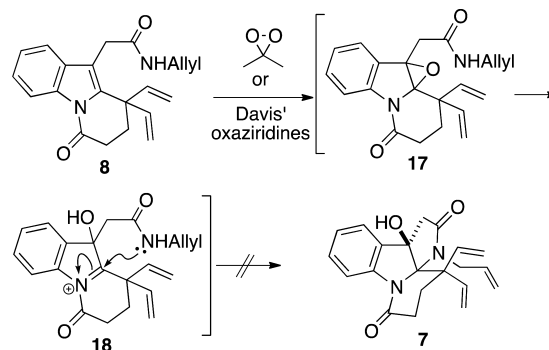
Scheme 4. Attempts for Oxidative Cyclization
