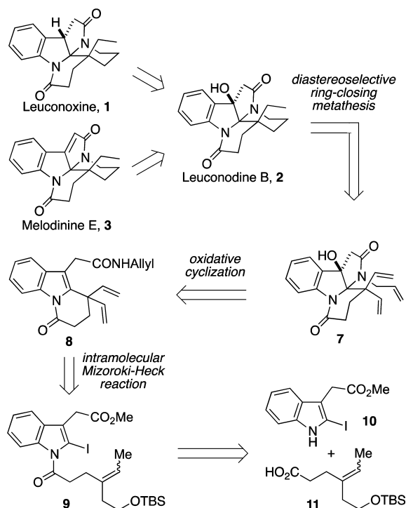
Scheme 2. Preparation of N -Acylindole 9
