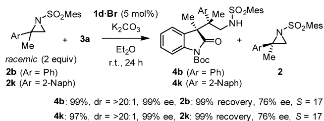
Scheme 1. Enantiomeric Excess of Recovered Aziridines 2 16
