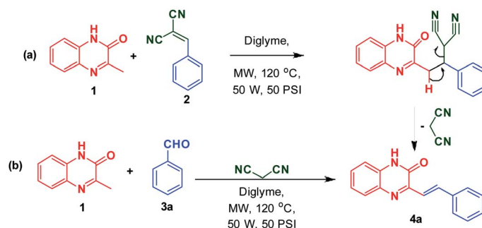
Scheme 2 (a) Synthesis of (E)-3-(4-methoxystyryl)quinoxalin-2(1H)-one 4a from 3MQ 1 and benzylidene malononitrile 2 ; (b) synthesis of (E)-3-(4-methoxystyryl)quinoxalin-2(1H)-one 4a from 3MQ 1 and aldehyde 3a .
