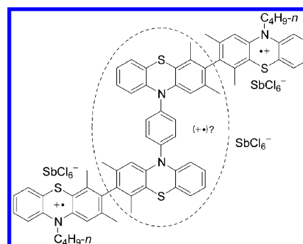
Figure 4. Potential structure of 1t(SbCl 6 ) 3 .
