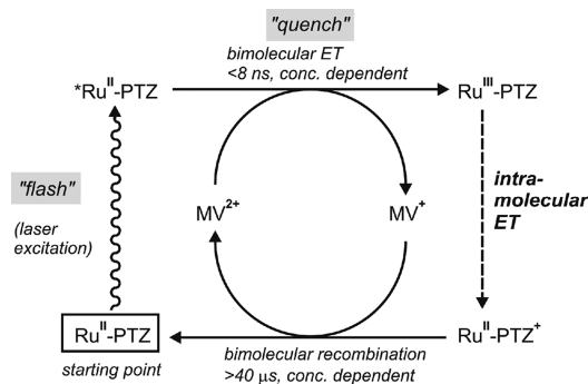
Scheme 3. Graphical Illustration of the Flash-Quench Technique Used for Phototriggering of Intramolecular Charge Transfer between Ru(III) and PTZ in the Ru–PTZ Dyad
