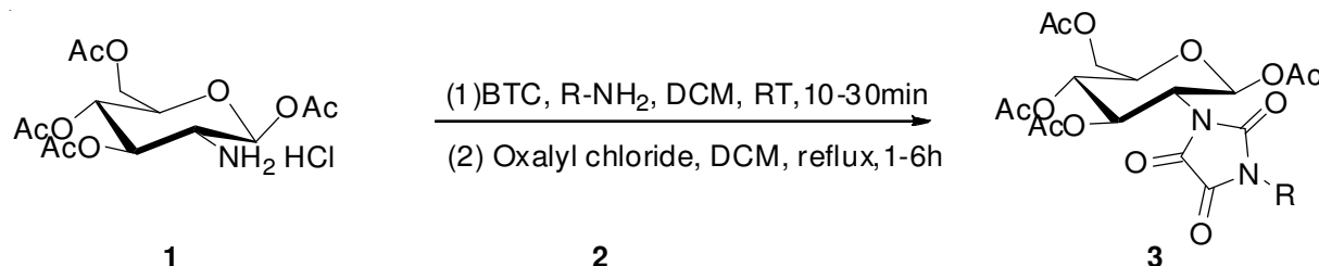
Scheme-I: Synthesis of the compounds 3
