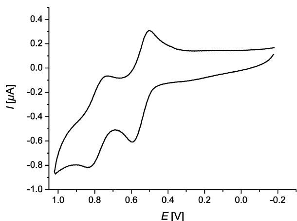
FIGURE 7. Cyclic voltammogram of 10 (recorded in dichloromethane, T = 293\text{ K} , \nu = 100\text{ mV/s} , electrolyte: \text{Bu}_4\text{N}^+ \text{PF}_6^- , Pt working electrode, Pt counter electrode, Ag/AgCl reference electrode).
