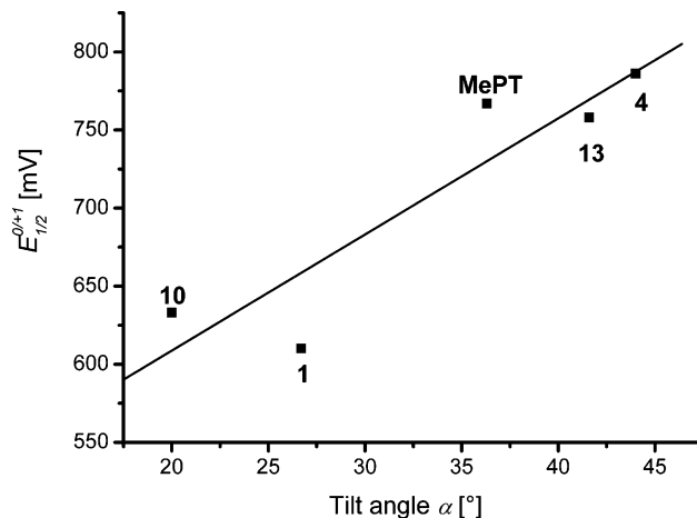
FIGURE 8. Linear fit of the tilt angles \alpha vs first oxidation potentials E_0^{0/+1} = 459.91 + 7.440\alpha\text{ [mV]} ( r^2 = 0.915 ).
