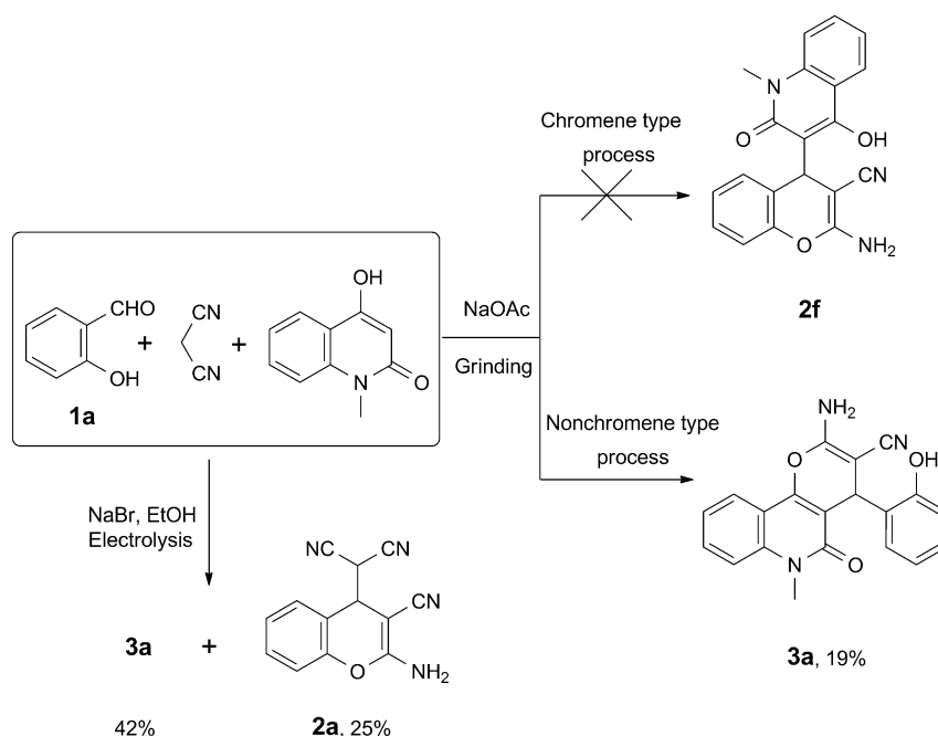
Scheme 2. Multicomponent Transformation of Salicylaldehyde 1a , Malononitrile, and 4-Hydroxy-1-methylquinolin-2(1H)-one on Solvent-Free and Electrocatalytic Conditions
