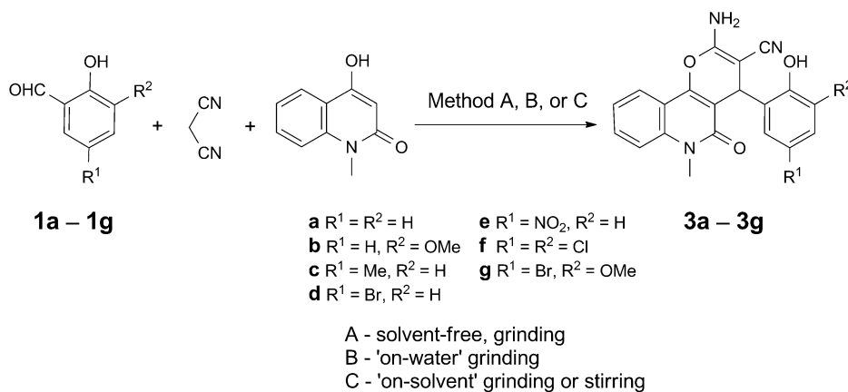
Scheme 3. Multicomponent Transformation of Salicylaldehydes 1a–1g , Malononitrile, and 4-Hydroxy-1-methylquinolin-2(1 H )-one into Pyrano[3,2- c ]quinolines 3a–3g
