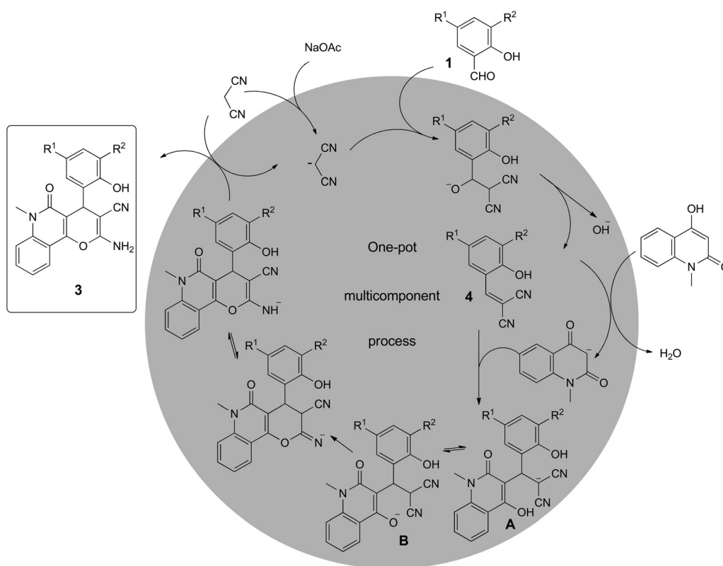
Scheme 4. Mechanism of Transformation of Salicylaldehydes 1 , Malononitrile, and 4-Hydroxy-1-methylquinolin-2(1H)-one into Substituted Pyran[3,2-c]quinolines 3
