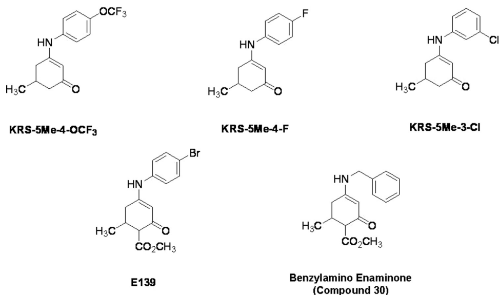
Fig. 2. Chemical structure of anilino enaminone analogs. The difference among the three mono methyl compounds is the anilino substitution represented by meta -chloro; para -fluoro, and para -trifluoro. E139 is a para -bromo anilino enaminone derivative with ortho -methyl ester substituted moiety at cyclohexenone, and compound 30 is the benzylamino analog.
