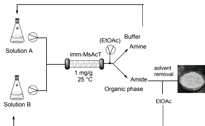
Scheme 1. Flow synthesis of amides. Solution A: 0.5 M or 1.0 M amine solution in phosphate buffer (0.1 M, pH 8.0) containing 5–10% DMSO. Solution B: EtOAc or vinylOAc. T= 25 °C, P= atmospheric pressure.
