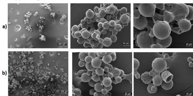
Figure 1. SEM images of agarose matrix particles. Line a: MsAcT immobilization 60x; 500x; 1000x magnification respectively. Line b: activated glyoxyl agarose after MsAcT immobilization (1 mg/g matrix ) 60x; 500x; 1000x magnification respectively.
