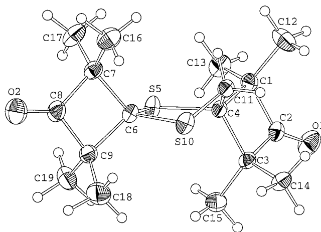
Figure 1. Structure of 1,3-dithiolane 4 (ORTEP plot; thermal ellipsoids at 30 % probability level) showing the envelope conformation of the heterocycle. Selected bond lengths [Å]: C4–S5 1.817(2), S5–C6 1.826(2), C6–S10 1.813(2), S10–C11 1.793(2), C11–C4 1.526(3), C3–C4 1.598(2), C6–C9 1.601(3); bond angles [ ^\circ ]: C4–S5–C6 100.37(9), S5–C6–S10 106.4(1), C6–S10–C11 95.04(9), S10–C11–C4 106.7(1), C11–C4–S5 104.3(1); dihedral angles [ ^\circ ] within heterocycle at: C4–S5 -27.6(2) , S5–C6 -4.9(1) , C6–S10 29.8(1) , S10–C11 -51.5(1) , C11–C4 51.4(1) .
