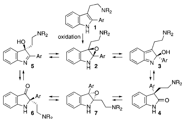
Scheme 1. Stereoselective Rearrangement of 2-Aryl Tryptamines
