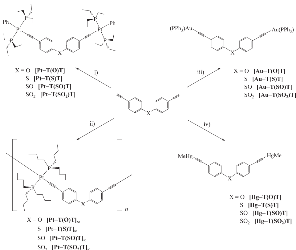
Scheme 2. Synthesis of the platinum(II), gold(I) and mercury(II) alkynyls. i) trans -[PtPh(Cl)(PEt 3 ) 2 ] (2 equiv), CuI, i Pr 2 NH, RT; ii) trans -[PtCl 2 (PBU 3 ) 2 ] (1 equiv), CuI, i Pr 2 NH, RT; iii) [Au(PPh 3 )Cl] (2 equiv), NaOH/MeOH, RT; iv) [MeHgCl] (2 equiv), NaOH/MeOH, RT.
