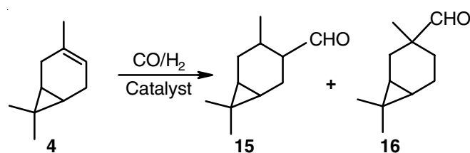
Scheme-IV: Hydroformylation of 3-carene
