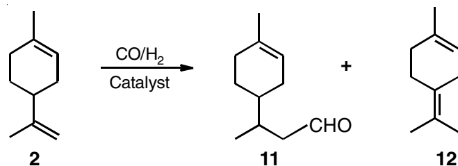
Scheme-II: Hydroformylation of limonene
