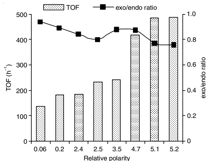
Fig. 1. A plot of activity and exo/endo ratio vs. relative polarity; Reaction conditions: camphene: 0.64 \text{ kmol/m}^3 , \text{Rh}(\text{CO})_2(\text{acac}) : 1.23 \times 10^{-3} \text{ kmol/m}^3 , \text{P}(\text{OPh})_3 : 7.4 \times 10^{-3} \text{ kmol/m}^3 (Rh:P = 1:6), T: 373 K, agitation speed: 16.6 Hz, \text{P}_{\text{CO}+\text{H}_2} : 4.14 MPa, total charge: 8.1 \times 10^{-5} \text{ m}^3 . % (hexane 0.06, cyclohexane 0.2, toluene 2.4, xylene 2.5, 1,2 DCE 3.5, MEK 4.7, methanol 5.1, ethanol 5.2)
