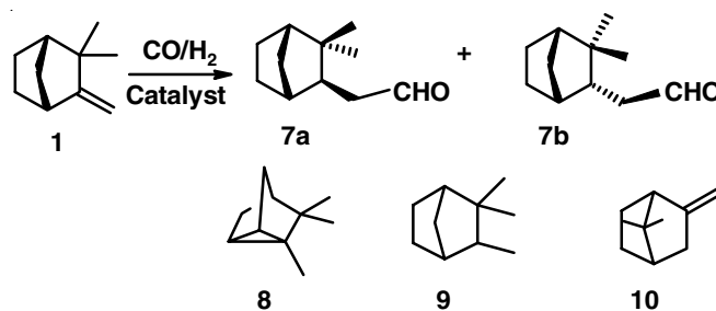
Scheme-I: Hydroformylation of camphene
