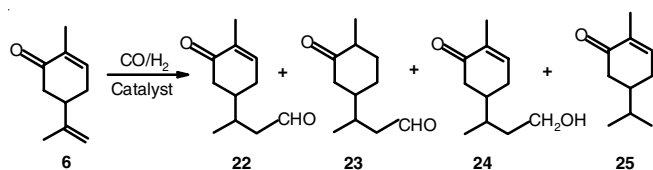
Scheme-VI: Hydroformylation of carvone
