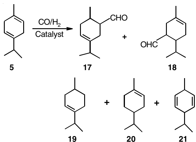
Scheme-V: Hydroformylation of \gamma -terpinene
