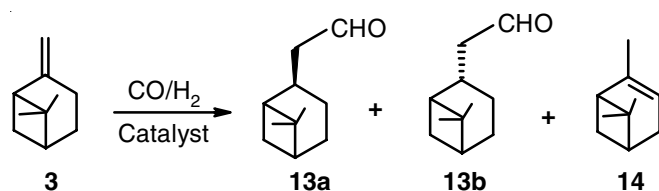
Scheme-III: Hydroformylation of \beta -pinene
