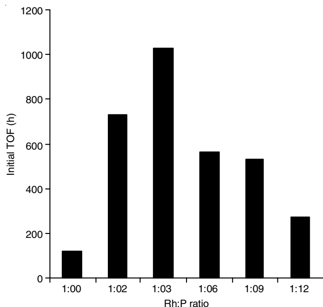
Fig. 2. A plot of initial activity vs. Rh:P ratio; Reaction conditions: \text{Rh}(\text{CO})_2(\text{acac}) : 1 \times 10^{-3} \text{ kmol/m}^3 , camphene: 0.37 \text{ kmol/m}^3 , T: 373 K, P_{\text{CO}+\text{H}_2} : 4.14 MPa, MEK: 2.82 \times 10^{-5} \text{ m}^3 , total charge: 3.0 \times 10^{-5} \text{ m}^3 , agitation speed: 16.6 Hz
