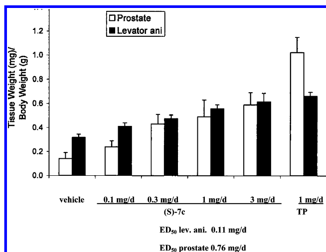
Figure 3. Effect of (S)-7c on levator ani and prostate weights in orchidectomized immature rats following oral administration ( p < 0.01 relative to vehicle, one-way ANOVA w/Dunnetts post-test, three rats per group, mean \pm SD).
