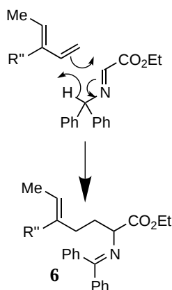
Scheme 4. Formation of ene by-product 6 from Table 1, entries 3/4 ( R''=H/Me ).
