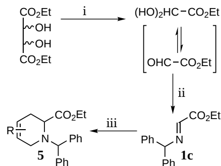
Scheme 3. Reagents and conditions: (i) \text{NaIO}_4 , \text{CH}_2\text{Cl}_2/\text{H}_2\text{O} 5:1, reflux, 1 h then cool to 0°C and add \text{MgSO}_4 (94%); (ii) \text{Ph}_2\text{CHNH}_2 (0.75 equiv.), \text{CH}_2\text{Cl}_2 , 3 Å MS, rt (94%); (iii) diene (2 equiv.), TFA (1 equiv.), TFE, –40°C (see Table 1, and Refs. 13–15 for experimental details and data).
