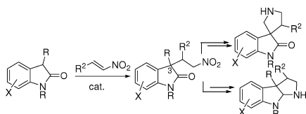
Figure 1. Synthetic route to oxindole derivatives.
