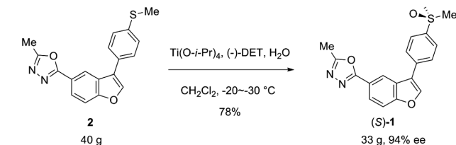
Chart 3. Scale-Up Synthesis of (S)-1
