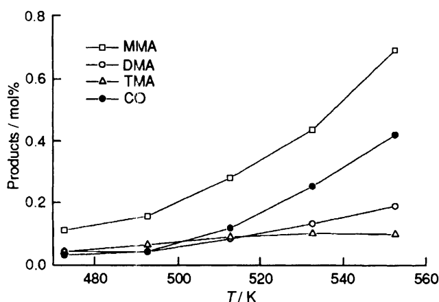
Fig. 1 Temperature dependence of formation of methylamines and CO over Cu–Al 2 O 3 . Conditions: 3 g catalyst (58.5 mass% CuO), 0.6 MPa, 150 cm 3 min −1 , CO 2 :NH 3 :H 2 , 1:1:3.
