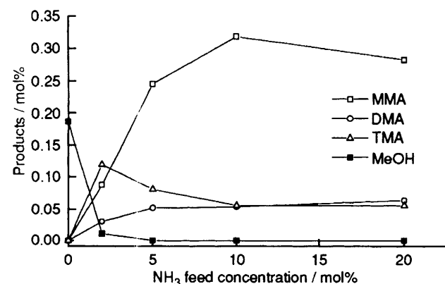
Fig. 2 Dependence of concentrations of methylamines and methanol on ammonia feed concentration. Conditions: 3 g catalyst (58.5 mass% CuO), 0.6 MPa, 513 K, 150 cm 3 min −1 , CO 2 :H 2 , 1:3.
