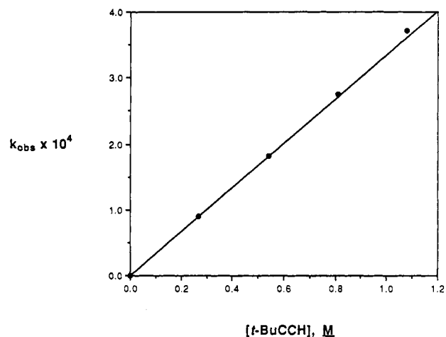
Figure 2. Linear dependence of k_{\text{obs}} on alkyne concentration at 50^\circ\text{C} .
