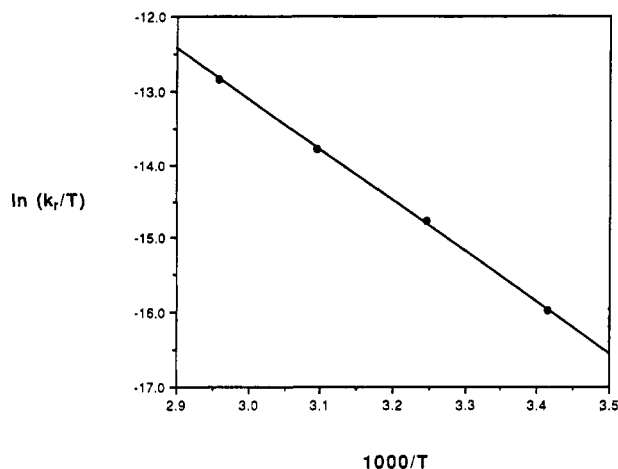
Figure 3. Eyring plot for the alkyne insertion reaction over the temperature range from 20 to 65 °C.
