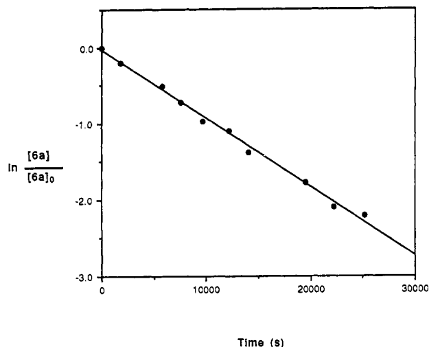
Figure 1. First-order plot for the conversion of 6a with t -BuCCH to 13b : [6a] = 0.017 M; [t\text{-BuCCH}] = 0.27 M; 50^\circ\text{C} .
