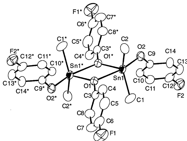
Fig. 2. ORTEP drawing of \text{Me}_2\text{Sn}(\text{OC}_6\text{H}_4\text{-p-F})_2 ( 2 ). Ellipsoids represent 50% probability.
