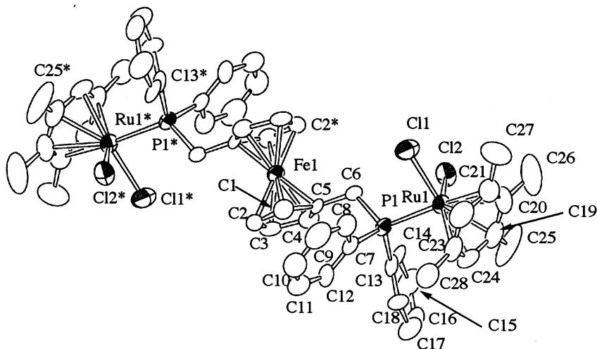
Fig. 2. Crystal structure of (\eta^6\text{-}1,2,3,5\text{-Me}_4\text{C}_6\text{H}_2)_2\text{Ru}_2\text{Cl}_4(\text{dppmf}) \cdot 2\text{CH}_2\text{Cl}_2 2d \cdot 2\text{CH}_2\text{Cl}_2 . Hydrogen atoms, solvated molecules and \text{PF}_6^- are omitted for clarity.
