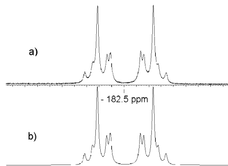
Figure 1. (a) Experimental ^{31}\text{P} NMR spectrum of 5 in toluene- d 8 (298 K) at 161.97 MHz, \delta -182.5 . (b) Simulated ^{31}\text{P} NMR spectrum of 5 (X part of the AA'XX' spin pattern: ^3J_{\text{H,H}} = 18.5 Hz, ^1J_{\text{P,H}} = 170.2 Hz, ^2J_{\text{P,H}} = 10.4 Hz, ^1J_{\text{P,P}} = 64.7 Hz).
