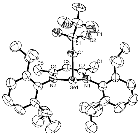
Figure 6. Molecular structure of 6 . Thermal ellipsoids are drawn at the 50% probability level. Hydrogen atoms are omitted for clarity. Selected bond lengths [Å] and angles [deg]: Ge1–N1 1.931(4), Ge1–N2 1.932(4), Ge1–O1 2.151(3), N1–C2 1.348(5), N2–C4 1.343(6), C2–C3 1.385(6), C3–C4 1.383(7), N1–Ge1–N2 93.0(2), N1–Ge1–O1 91.8(1), N2–Ge1–O1 89.7(1), C2–N1–Ge1 122.8(3), C4–N2–Ge1 123.3(3), N1–C2–C3 122.5(5), C4–C3–C2 127.3(4), N2–C4–C3 122.9(4).
