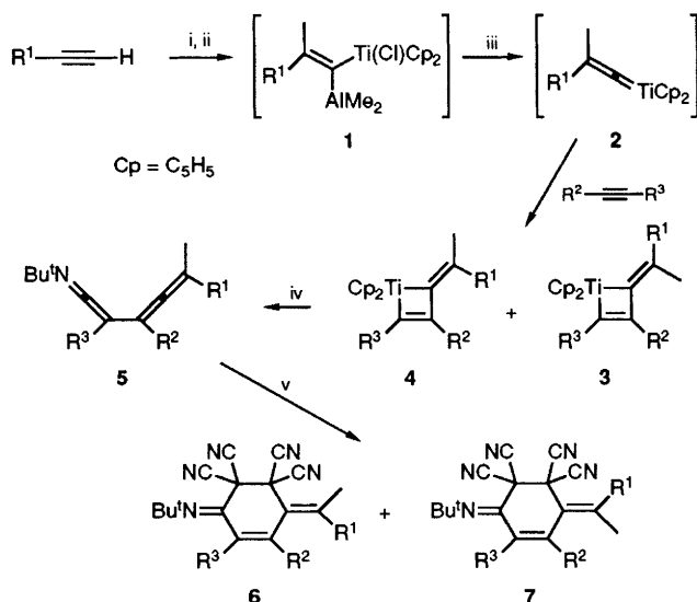
Scheme 1 Reagents and conditions: i, BuLi, 20°C, 15 min; ii, Cp 2 TiMeCl, Me 2 AlCl, toluene, 20°C, 2 h; iii, HMPA, 20°C, 15 min; iv, Bu t NC, hexane, 16 h, room temp.; v, TCNE, CHCl 3 , 0°C, 30 min
