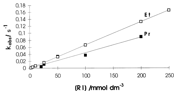
Fig. 3. Plot of k_{\text{obs}} versus [\text{RI}] ( \text{R} = \text{Et} or \text{Pr} ) for reaction (1), in THF at 25^\circ\text{C} . Concentration of complex (1) = 1.0 \times 10^{-4} M.
