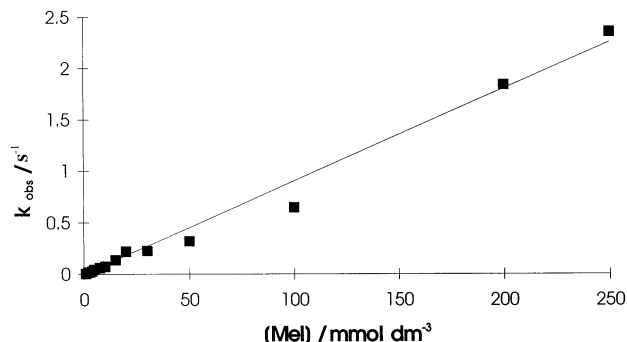
Fig. 2. Plot of k_{\text{obs}} versus [\text{MeI}] for reaction (1), in THF at 25^\circ\text{C} . Concentration of complex (1) = 1.0 \times 10^{-4} M.
