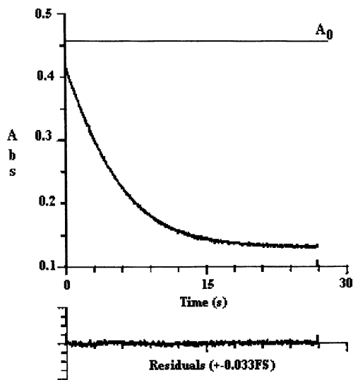
Fig. 1. Absorbance versus time dependence for the reaction of [\text{NBu}_4][\text{trans-Re}(\text{CN})_2(\text{dppe})_2] (1) ( 1.0 \times 10^{-4} M) with \text{MeI} ( 1.0 \times 10^{-1} M), in THF at \lambda = 400 nm, temperature = 25^\circ\text{C} ; A_0 , absorbance of complex (1). Curve was fitted using k_{\text{obs}} = 0.649 s ^{-1} , \Delta A = -0.31 , A_\infty = 0.13 , the residuals are shown at the bottom.
