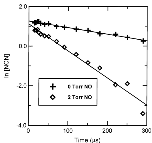
Figure 1. NCN laser-induced fluorescence signals as a function of time. Reaction conditions: P_{\text{CH}_2\text{N}_2} = 0.05 Torr, P_{\text{C}_2\text{N}_2} = 0.2 Torr. 193 nm photolysis.
