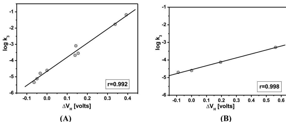
Figure 9. Plots of third-order experimental rate constants log k 3 (taken from ref 2) for the aminolysis of substituted phenyl N -phenylcarbamates with EPN values for the NH hydrogen atoms (Δ V H = V H (R) – V H (H)): (A) series 1 and (B) series 2 from Scheme 2.
