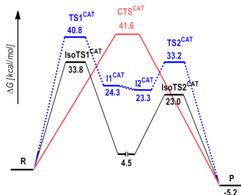
Figure 4. Energy diagram for the catalyzed aminolysis of phenyl N -phenylcarbamate along the concerted, addition–elimination stepwise, and isocyanate pathways from IEFPCM/M06-2X/6-311+G(2d,2p) computations.
