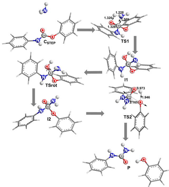
Figure 2. IEFCPCM/M06-2X/6-311+G(2d,2p) optimized structures along the stepwise mechanism via a tetrahedral intermediate for the aminolysis of phenyl N -phenylcarbamate.
