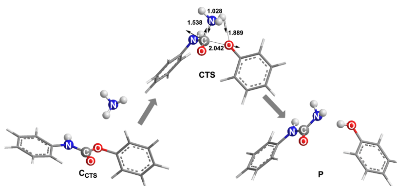
Figure 1. IEFCPCM/M06-2X/6-311+G(2d,2p) optimized structures along the concerted aminolysis of phenyl N -phenylcarbamate.
