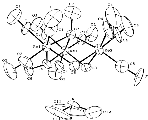
Fig. 1. Crystal structure of [\text{Me}_3\text{NH}]^+[\text{Re}_3(\text{CO})_9(\mu\text{-OH})_2(\mu\text{-OMe})(\mu_3\text{-OMe})]^- , 3 .
