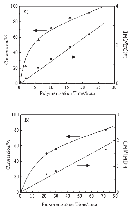
Figure 2. The first-order kinetic plots of the polymerization of A) monomer 5 with the feed ratio of [\mathbf{M}]_0/[\mathbf{I}]_0 of 100 and B) 6 with the feed ratio of 20 by the \mu -ethynediyl Pd–Pt dinuclear complex as the initiator in THF heated under reflux.
