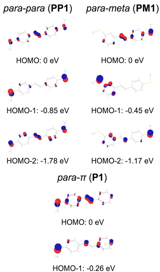
Figure 5. DFT calculated isosurfaces of MOs relevant in single-molecule conductance. Geometries of PP1, PM1, and P1 were optimized and MOs calculated at the B3LYP/6-31** level of theory in the gas phase. HOMO energies were normalized to 0 eV for easy comparison. Contour values set at 0.75.
