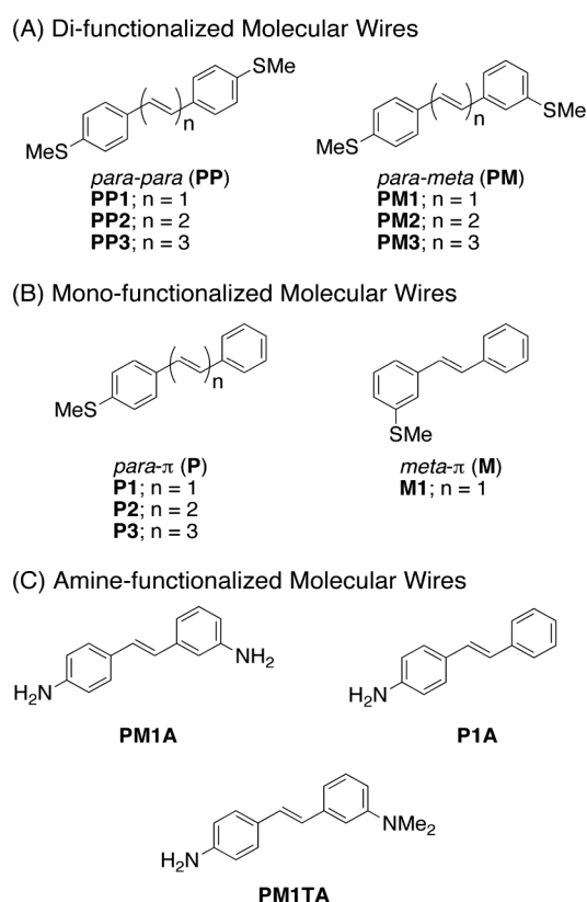
Figure 1. Chemical structures of trans -stilbene and all- trans -oligoene molecular wires: (A) difunctionalized series, having only para -positioned linker groups (PPn) or a mixture of para and meta linkers (PMn); (B) monofunctionalized wires Pn and M1 contain either one meta or one para linker. (C) Stilbene derivatives end-functionalized with primary and tertiary amines.
