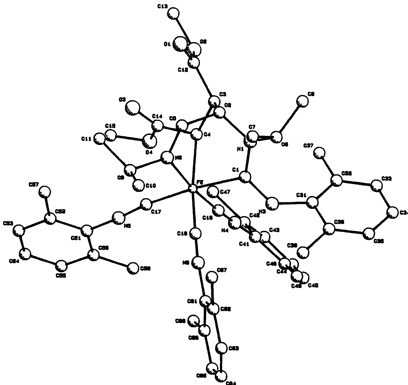
Figure 1. PLUTO drawing of \text{Fe}(\text{2,6-xylylNC})_3[\text{2.2.2}] \text{bic} (7a). Hydrogen atoms were left out for clarity.
