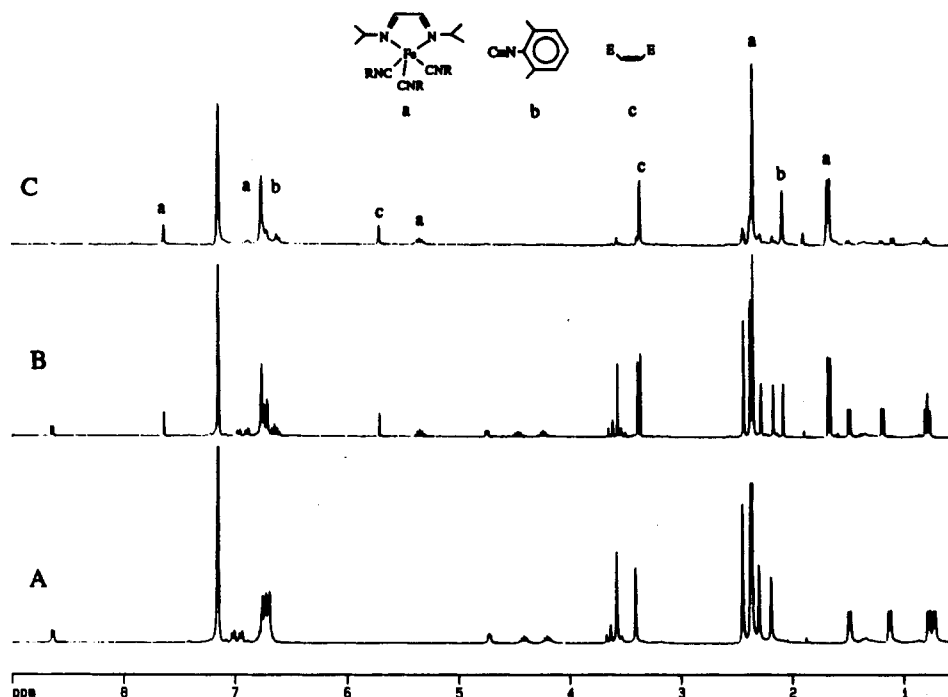
Figure 4. 1 H NMR spectra, recorded in C 6 D 6 at 333 K within ca. 1.5 h, showing the disassembly of Fe(2,6-xylylNC) 3 [(2.2.2)bic] (7a) (spectrum A) to its starting components 34 (spectrum C).
