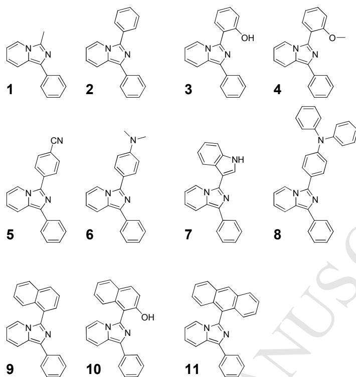
Fig. 1. 3-substituted-1-phenylimidazo[1,5- a ]pyridines.
