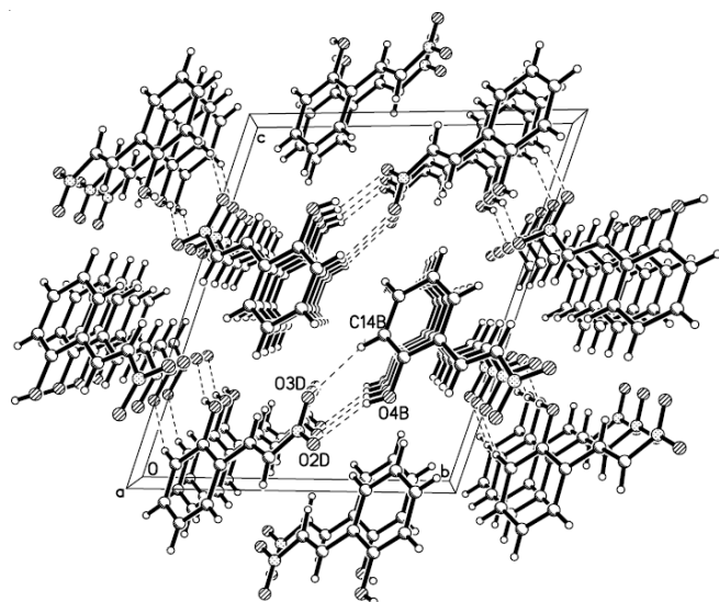
Fig. 3. Crystal packing diagram of (I) along the a -axis
