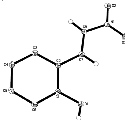
Fig. 2. Molecular structure of ( I ) with 30 % probability thermal ellipsoids
