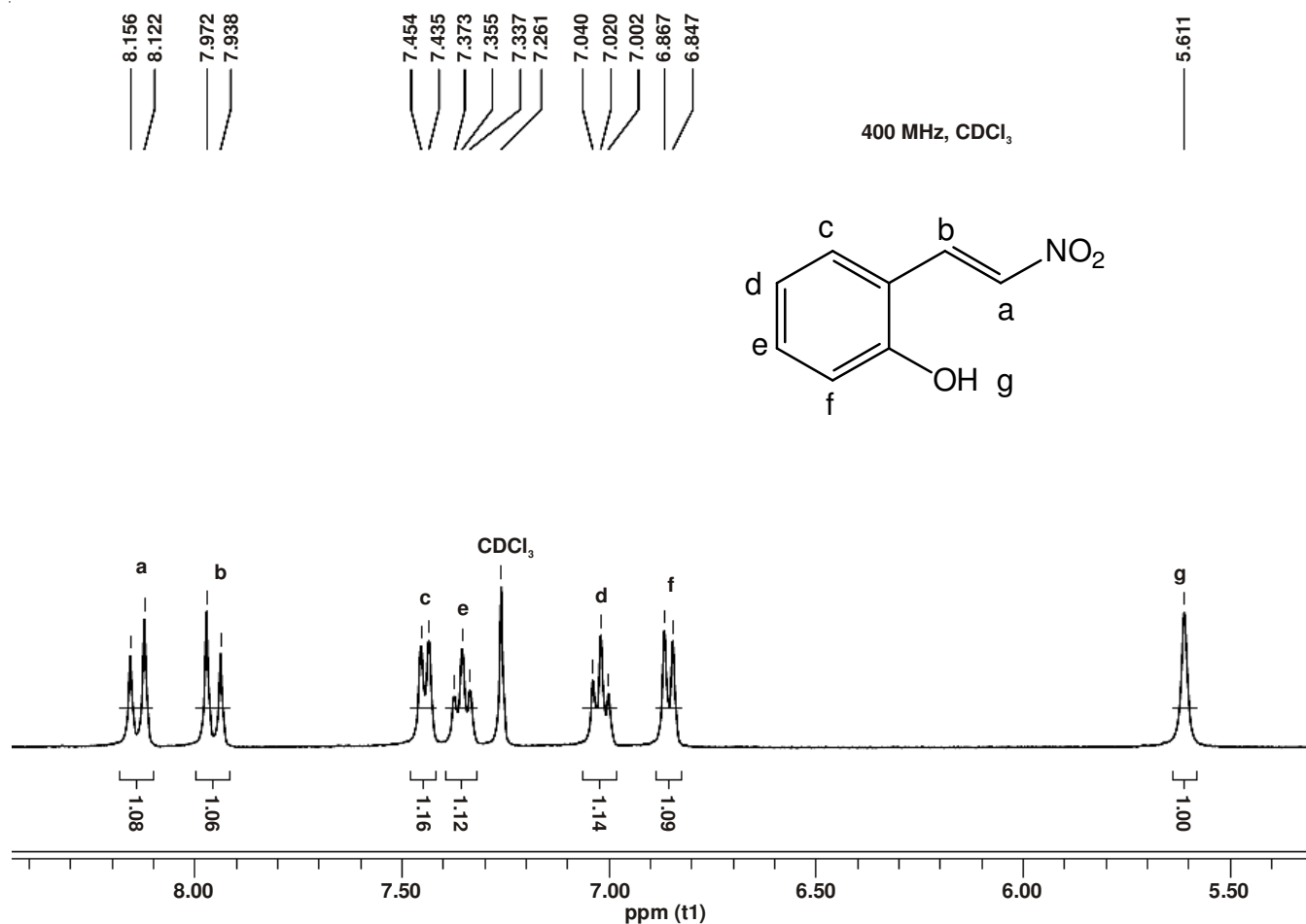
Fig. 1. 1 H NMR spectrum of ( I )
