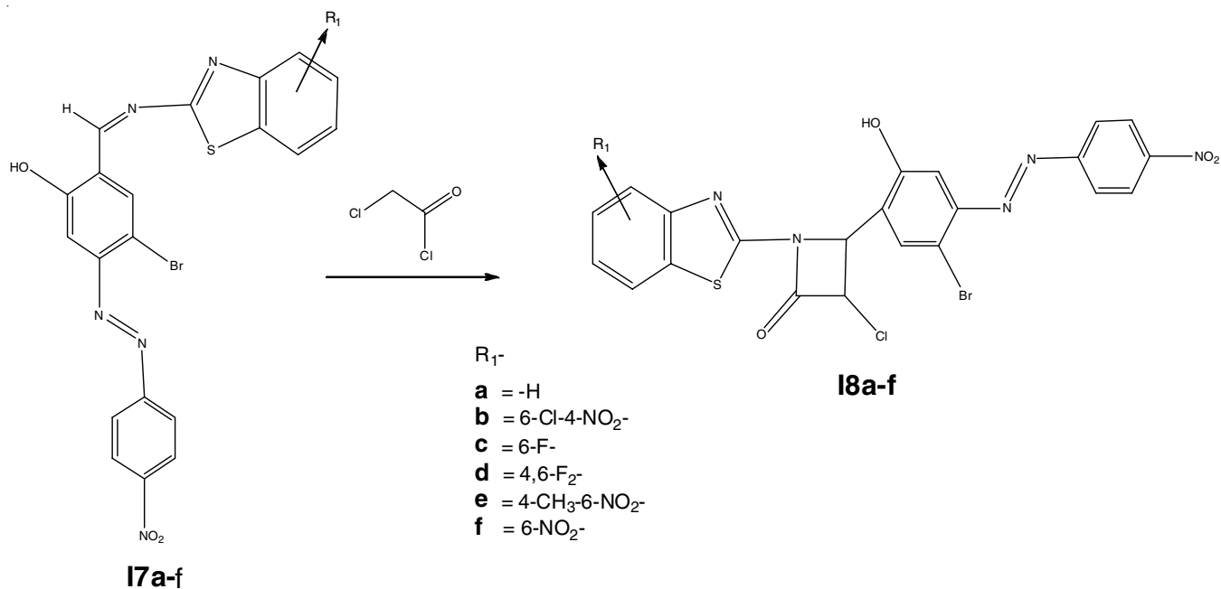
Scheme-II: Synthesis of \beta -lactam derivatives
