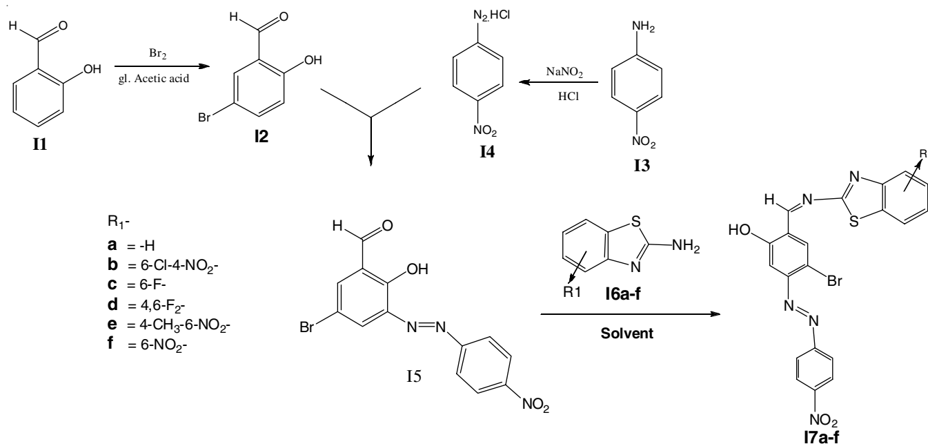
Scheme-I: Synthesis of azo Schiff bases
