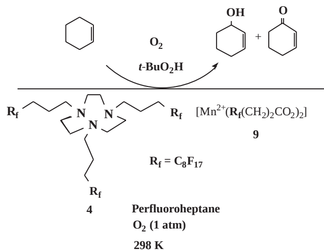
Scheme 2. Fluorous biphasic oxidation catalysis with cyclohexene as the substrate and complex 11 formed in situ from 4 and 9 .
