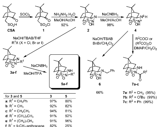
Scheme 1. Preparation of the Camphor Sulfonyl Hydrazines (CaSH)
