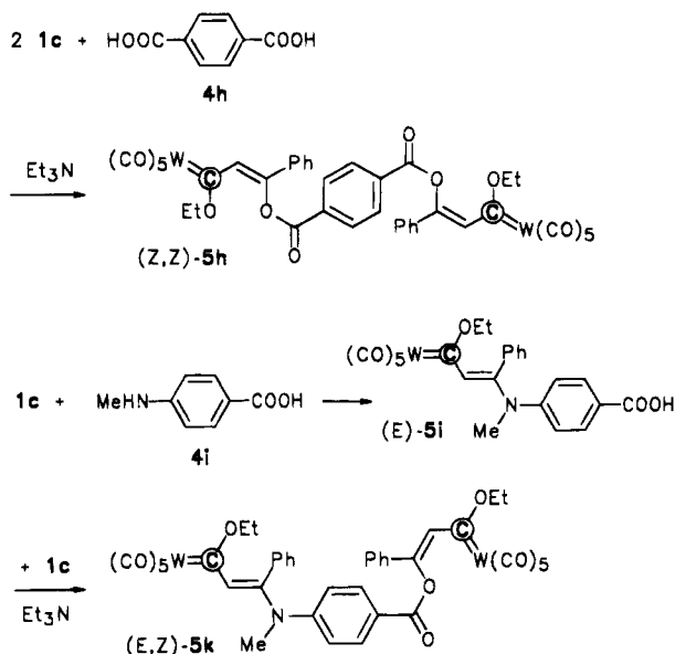
Scheme 6. Bis(carbene) Complexes (Z,Z)-5h and (E,Z)-5k
