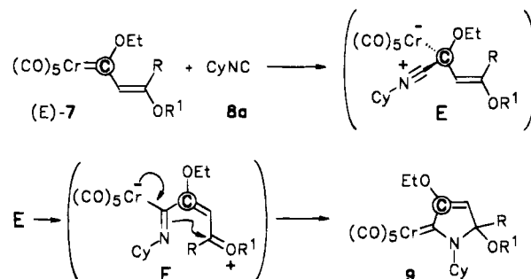
Scheme 4. 4,5-Dihydropyrrolylidene Complexes 9 by Cyclization of (2-Alkoxyethenyl)carbene Complexes (E)-7 with 8a
