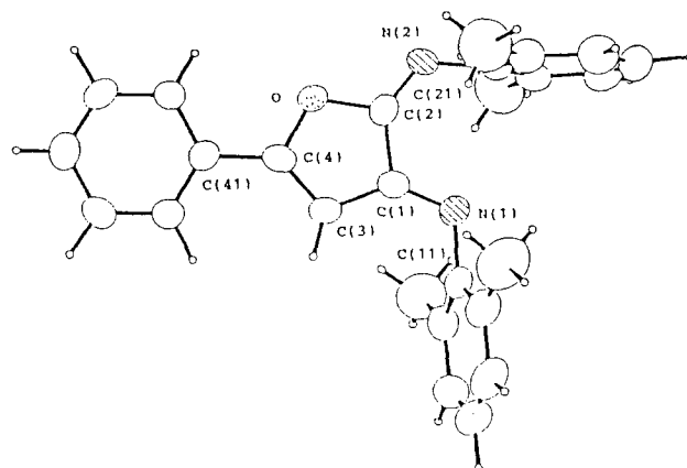
Fig. 1. Structure of 1a .
