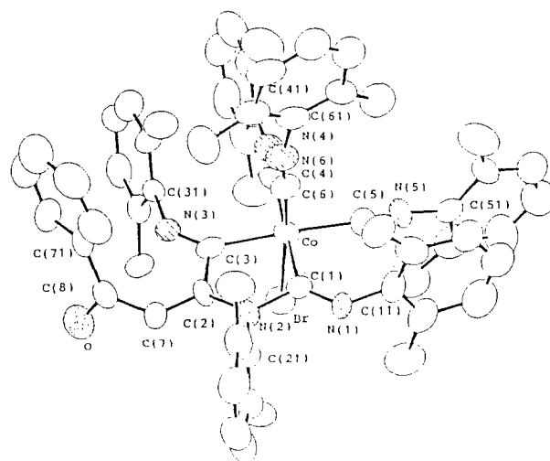
Fig. 2. Structure of 2a .
