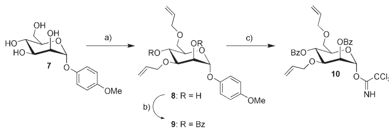
Scheme 2. Synthesis of the allylated mannosyl donor 10 . a) i) Bis(tributyltin)oxide, toluene, reflux, 4 h; ii) \text{AlBr}_3 , \text{TBABr} , 80^\circ\text{C} , 7 d, 51 %; b) \text{BzCl} , pyridine, 0^\circ\text{C} \rightarrow \text{RT} , overnight, quant.; c) i) \text{CAN} , \text{MeCN}/\text{H}_2\text{O} (4:1), 0^\circ\text{C} \rightarrow \text{RT} , 3 h; ii) trichloroacetimidate, \text{CH}_2\text{Cl}_2 , \text{DBU} , 0^\circ\text{C} \rightarrow \text{RT} , 1 h, 53 % (over two steps).
