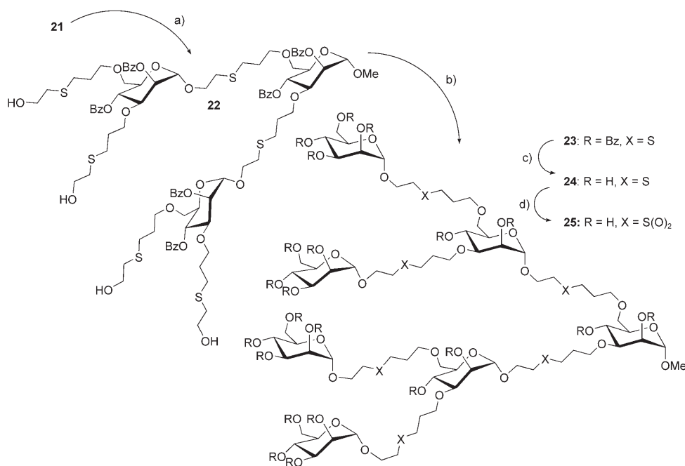
Scheme 6. Glycodendron synthesis with mercaptoethanol addition. a) \text{HS}(\text{CH}_2)_2\text{OH} , AIBN, dioxane, 75^\circ\text{C} , 4 h, 94 %; b) 4 , TMSOTf, \text{CH}_2\text{Cl}_2 , RT, overnight, 55 %; c) NaOMe, MeOH/MeCN, RT, 68 %; d) MMPP, \text{H}_2\text{O}/\text{MeOH} overnight, RT, 67 %.
