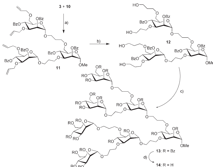
Scheme 3. Synthesis of the pseudo-heptasaccharide glycodendron 14 . a) \text{TMSOTf} , \text{CH}_2\text{Cl}_2 , RT, overnight, 79 %; b) i) 9-BBN, THF, reflux, 1 h; ii) 3 M \text{NaOAc} (aq.), \text{H}_2\text{O}_2 (30 %), 0^\circ\text{C} \rightarrow \text{RT} , overnight, 40 %; c) 4 , \text{TMSOTf} , \text{CH}_2\text{Cl}_2 , RT, overnight, 54 %; d) \text{NaOMe} , \text{MeOH} , RT, 88 %.
