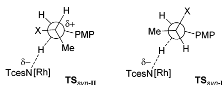
Figure 3. Transition states TS syn-II and TS syn-I of a diastereoselective amination reaction evolving from two of the conformations depicted in Figure 2.
